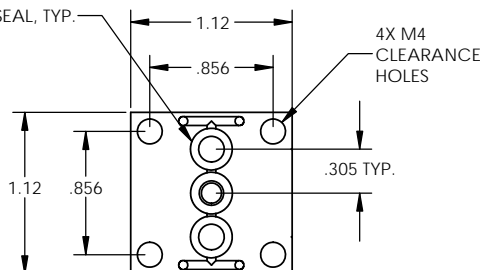
3-PORT, CENTER
